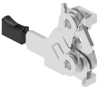
手动驱动 (图示为左侧单级型) Hand Actuation (left hand, single stage version shown)
