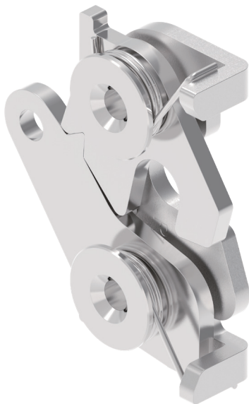
远程驱动 (图示为左侧双级型) Remote Actuation (left hand, two stage version shown)
