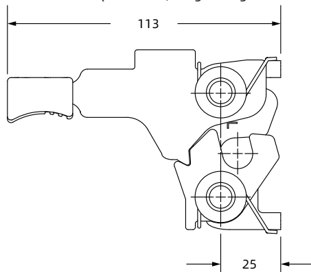
手动驱动 (图示为左侧单级型) Hand Actuation (left hand, single stage version shown)
