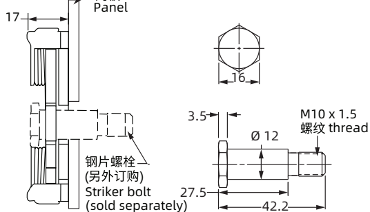
钢片螺栓 (另外订购) Striker Bolt (sold separately)
