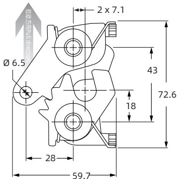
远程驱动 (图示为左侧双级型) Remote Actuation (left hand, two stage version shown)
